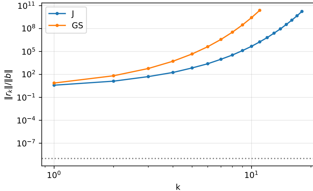
chebvand, n = 5
